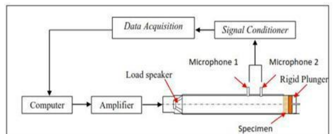
Drawing 2. Impedance tube installation
