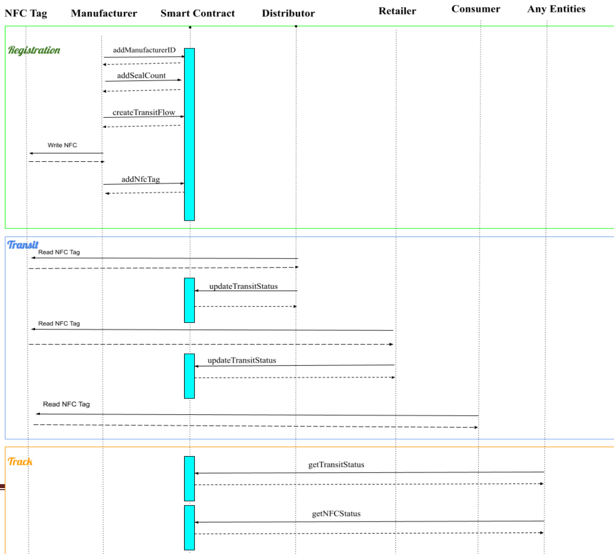
Figure 4 Sequence diagram representing end to end workflow
