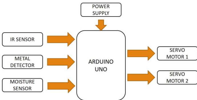
Fig 10: Block Diagram
