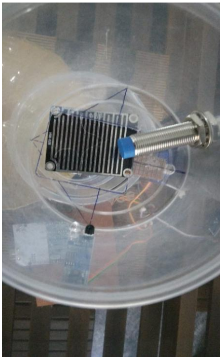
Fig 13: Metal sensor and Wet sensor are attached
