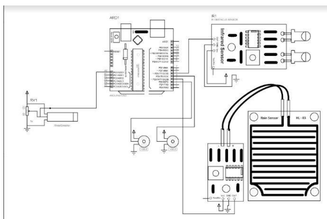
Fig 11: Circuit Diagram
