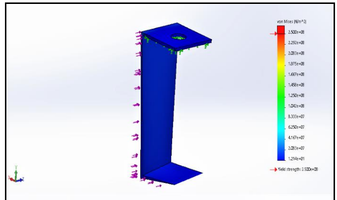
Fig -10: Result of the stress analysis of optimized blade of weeding tool
