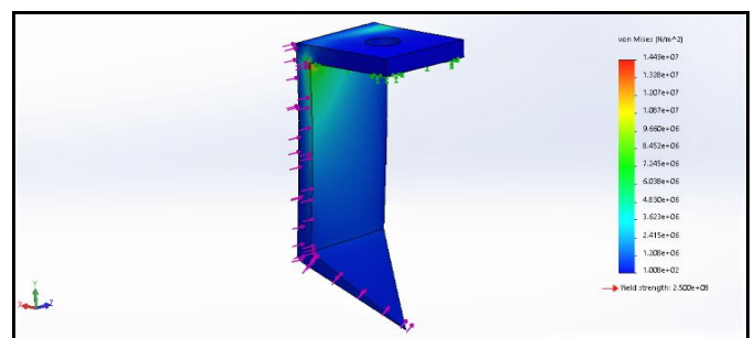
Fig -5: Result of Static stress analysis of a blade
