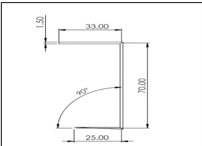
Fig -9: Front view of optimized blade of the tool
