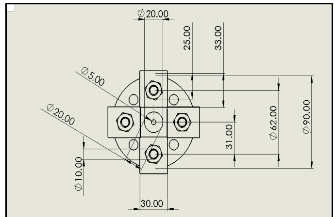
Fig -7: Top view of manufactured weeding tool
