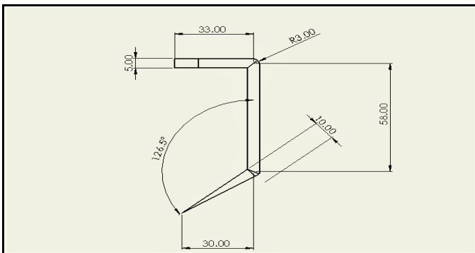
Fig -3: Front view of blade
