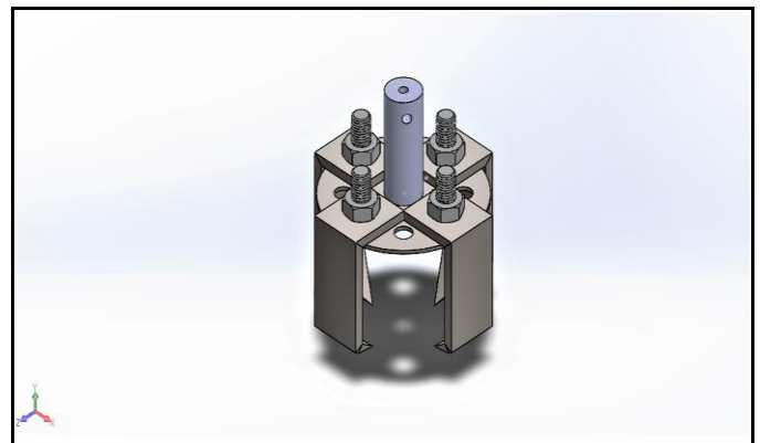
Fig -1: Weeding tool assembly (Without motor)
