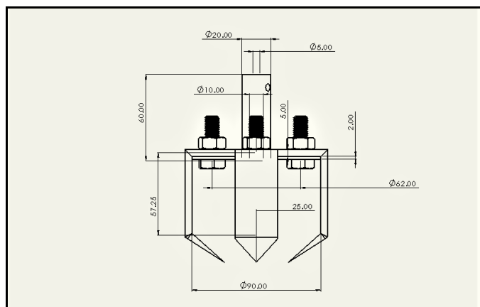
Fig -6: Front view of manufactured weeding tool
