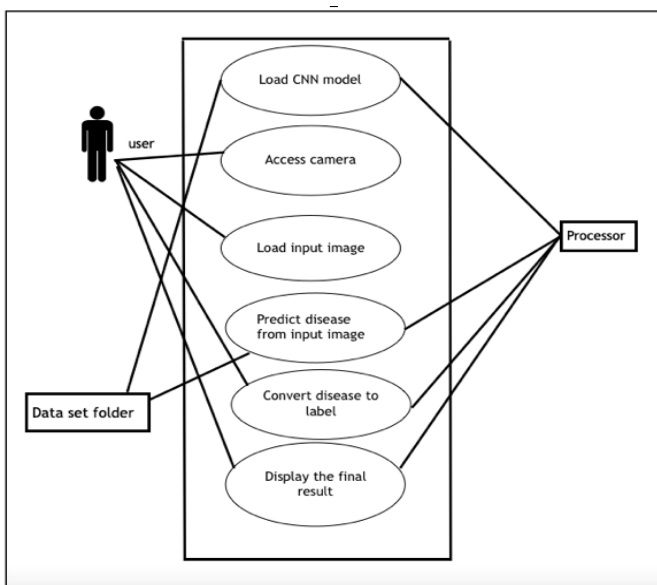
Fig -2: Interaction among different functions of the project
