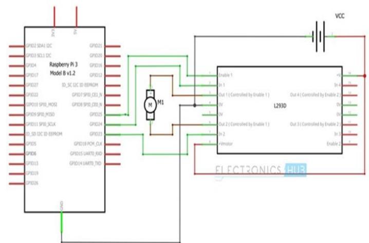
Fig -5: Circuit Diagram of Motor Interfacing with L293D
