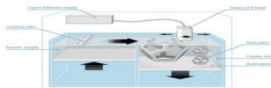
Figure 1 Binder Jetting Machine
