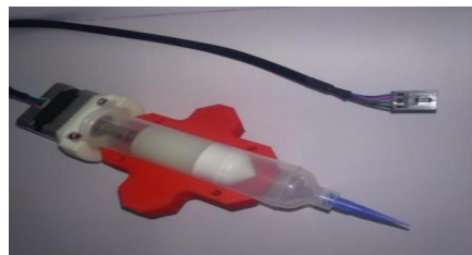
Figure 4 Binder Extrusion Head
