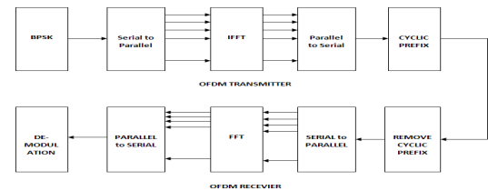
Fig.3 Block diagram of OFDM Transmitter and receiver.
