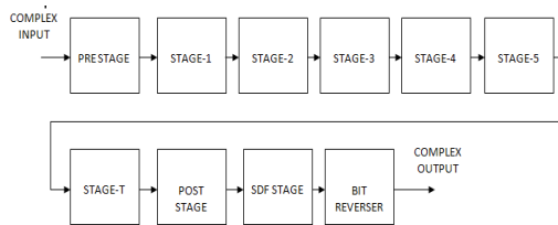
Fig.4 Proposed system block diagram.
