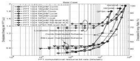
Fig.6 FFT radix
