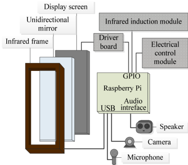
Fig-1: Hardware Architecture
