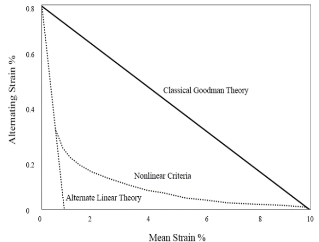
Figure 3: Modified Goodman diagram may be used to analyze the effects of mean strains on fatigue lifetime NiTi.
