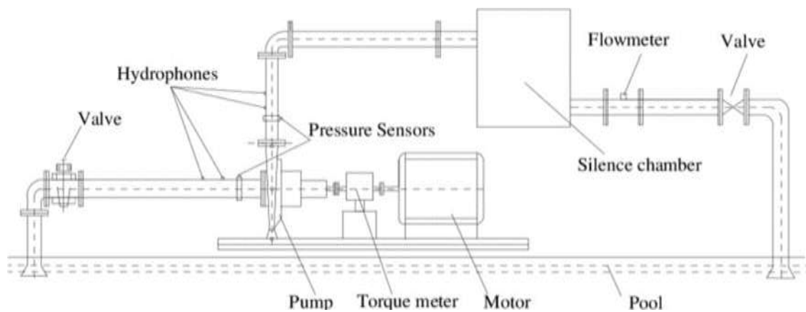
Fig. 1. Pump System centrifugal pump
