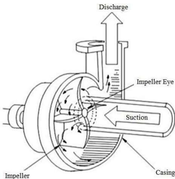
Fig. 2. Section view of Centrifugal Pump
