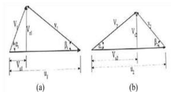
Fig. 5. Virtual Velocity Diagrams of Impeller (a) virtual inlet velocity, (b) virtual outlet velocity
