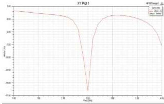
Fig.4 Return loss (S 11 ) parameter of the E-shape microstrip patch antenna
