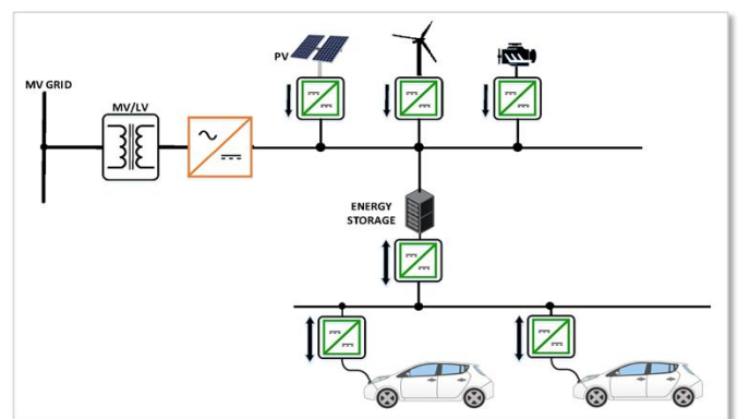
Figure : 1 Proposed Method for EV Charging Station integrated with Renewable Sources
