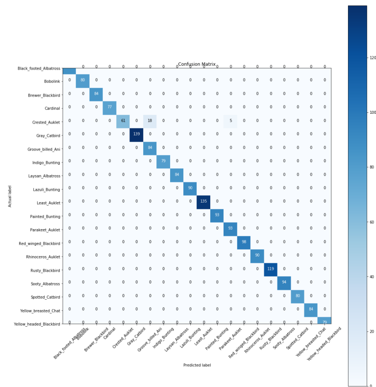
Figure 2. The confusion matrix for the classification model.
