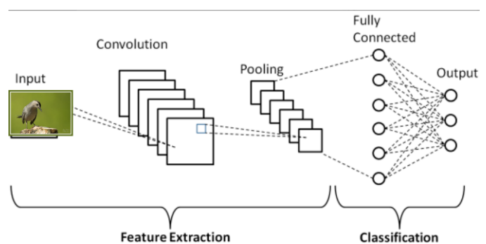
Figure 1. The Convolution neural network model for bird's species classification.
