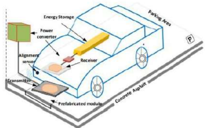
fig :2 Static wireless ev charging
