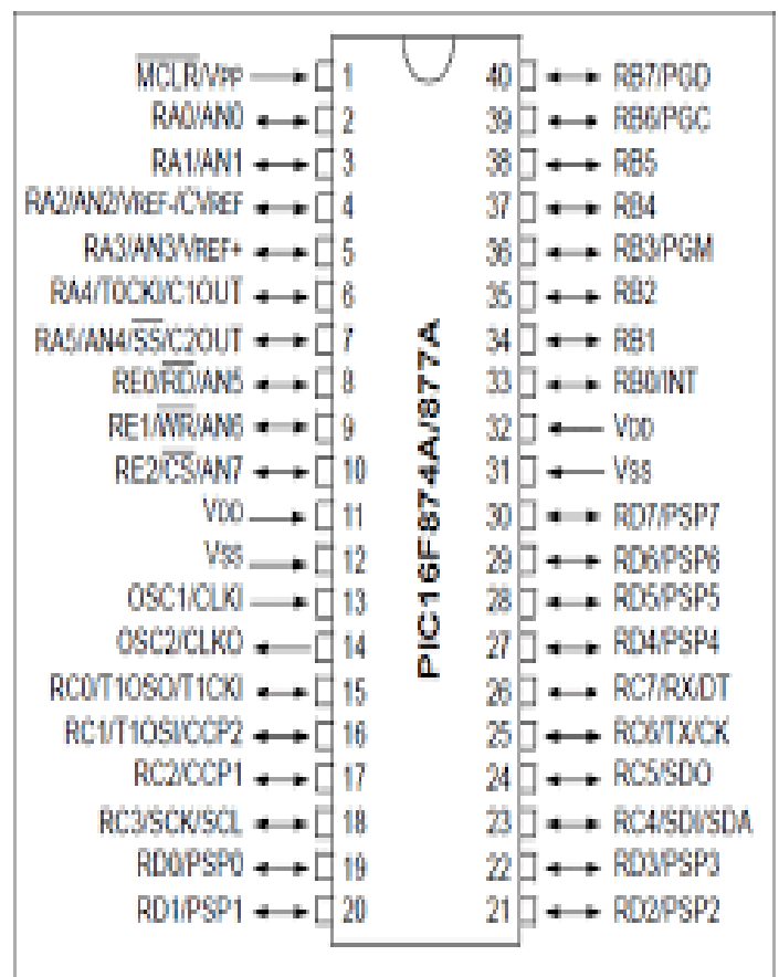
Fig.3: Pin Diagram of a PIC 16F876
