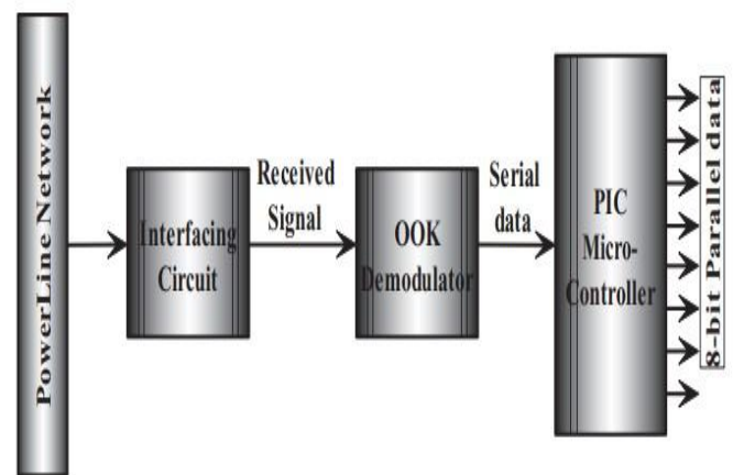
Fig.5: A block diagram of the proposed PLC receiver.
