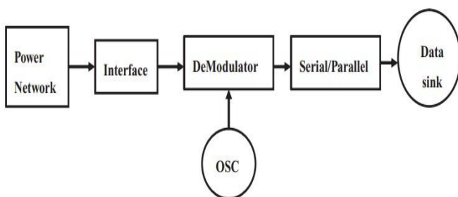
Fig.2: Block Diagram of PLC Reciever System
