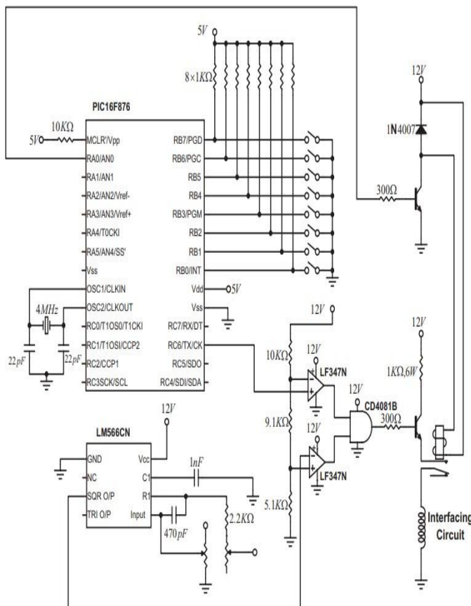
Fig.4: PLC transmitter schematic
