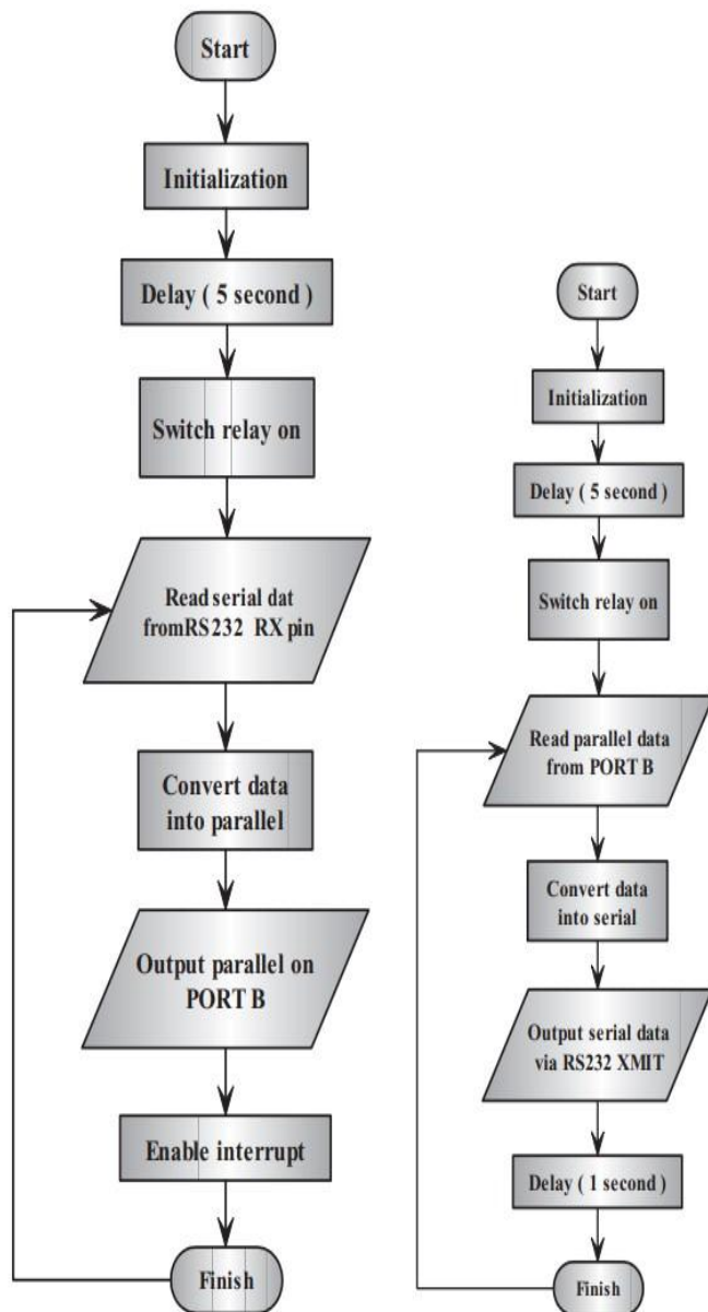
Fig.6: Flow chart used to program the PIC-16F876.
