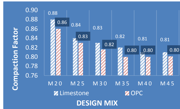
Workability test for 30% Replacement
