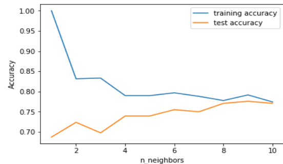
Figure 6: Training and Test accuracy in K-neighbors (Histogram)
