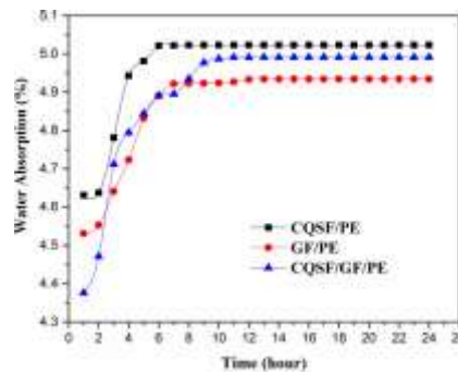
Fig. 1. Water absorption properties of composites
