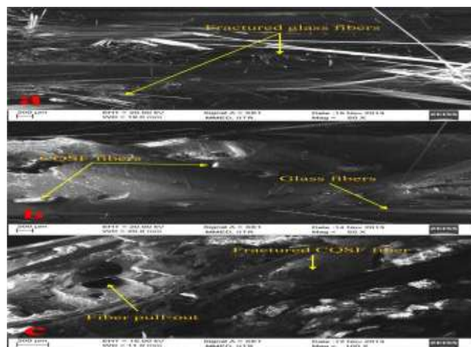
Fig.2. (a) Glass fiber/PE, (b) Glass fiber/CQSF/PE, (c) CQSF/PE
