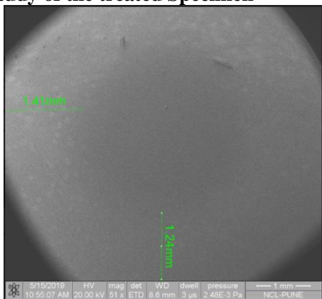
Fig.1 shows the SEM result in which carburizing occurred up to the 1.41 & 1.24 mm from the surface of specimen
