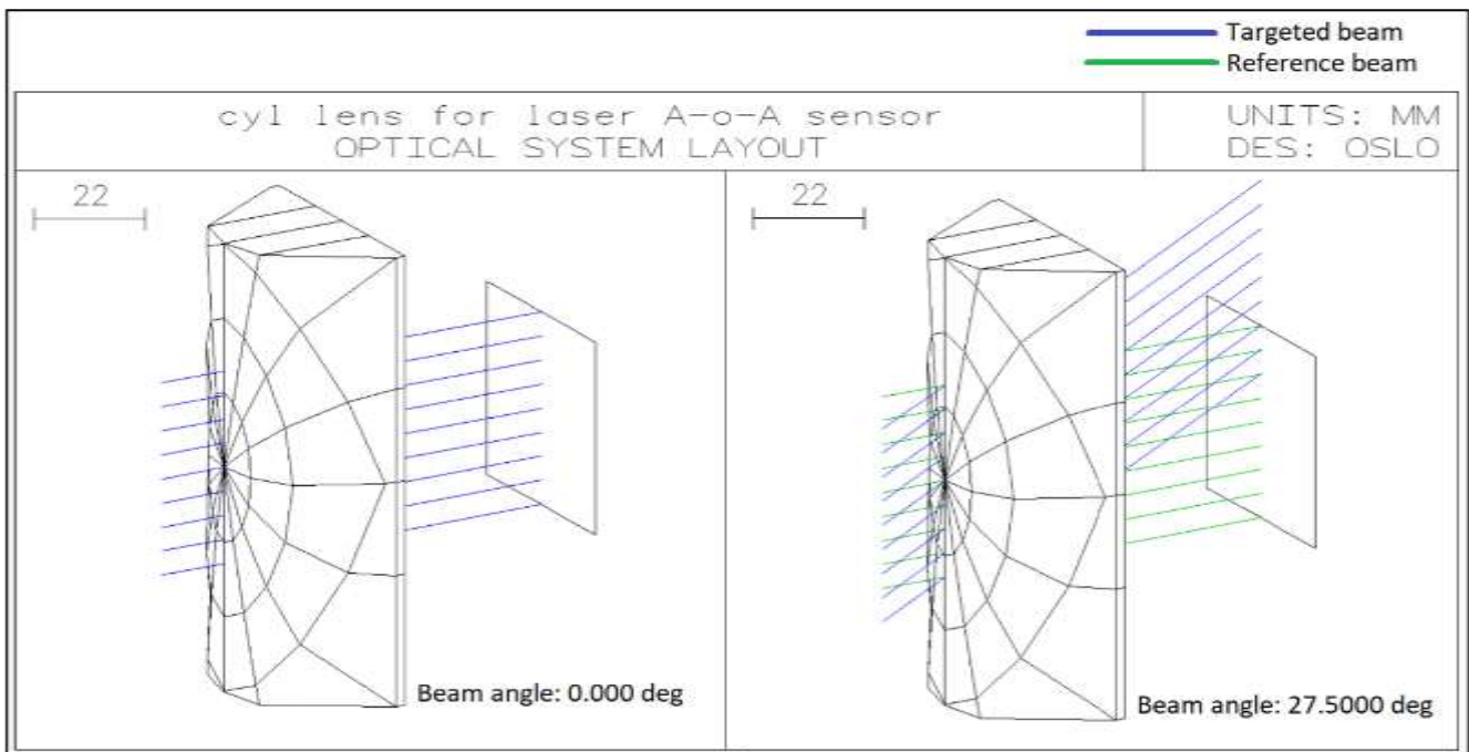
Fig - 4: Cylindrical lens showing the beam tilt and focusing of the beam at 0° angle-of-arrival (left) and at 27.5° angle-of-arrival (right) of the incident Laser beam
