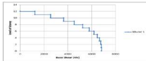
Base Shear diagram for model 1 along longitudinal direction.
