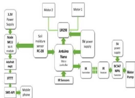
Fig-5: SYSTEM ARCHITECTURE
