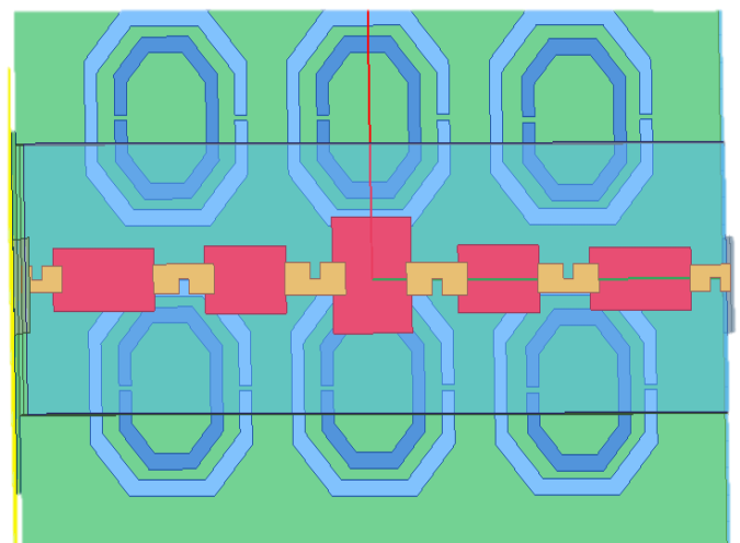
Fig 3. Linear array with CSRR structure
