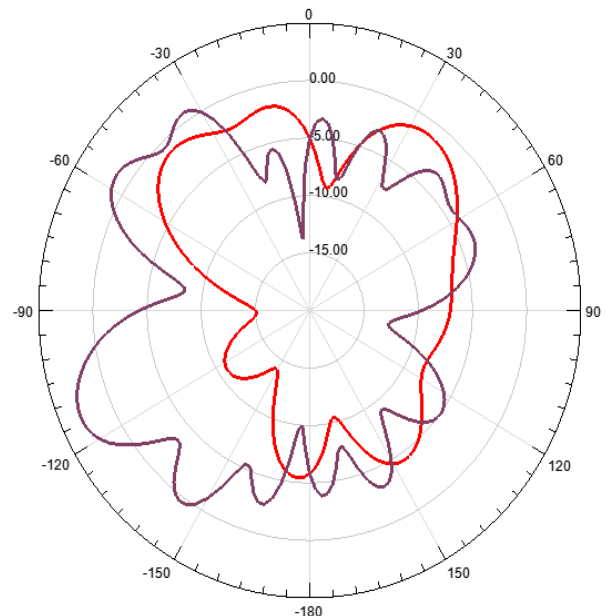
Fig 6(a). 2D gain plot
