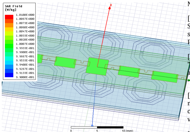
Fig 7. Simulation result of SAR value measurement
