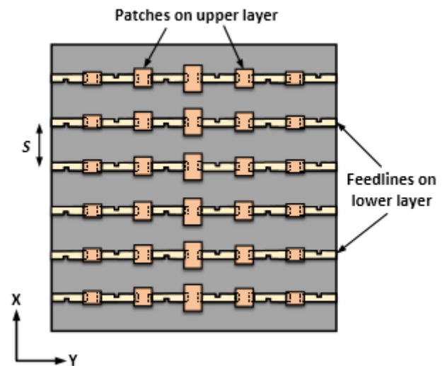
Fig 2. planar array configuration
