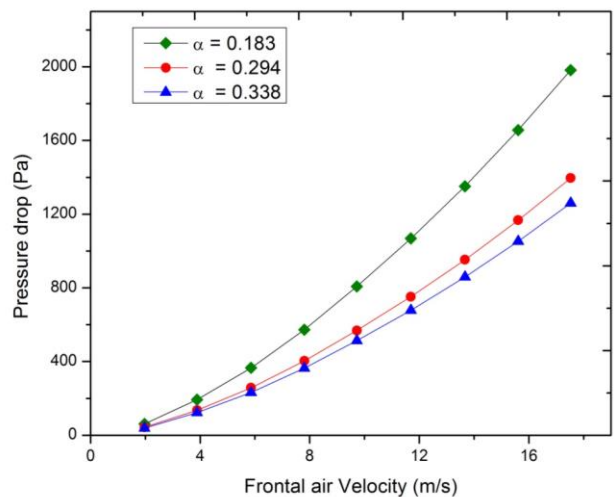
Fig.4. Pressure drop (ΔP) versus frontal air velocity (V) with different values of alpha (α).
