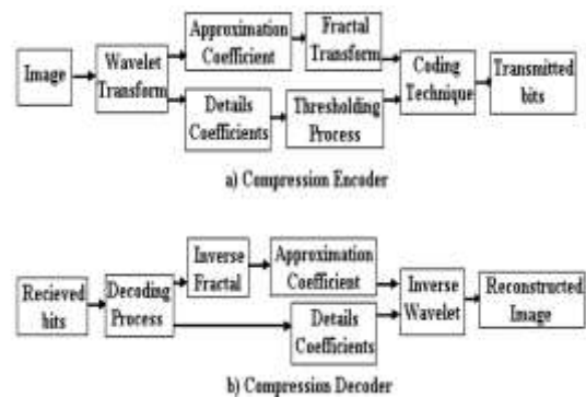
Fig: 1 Block Diagram of FIC
