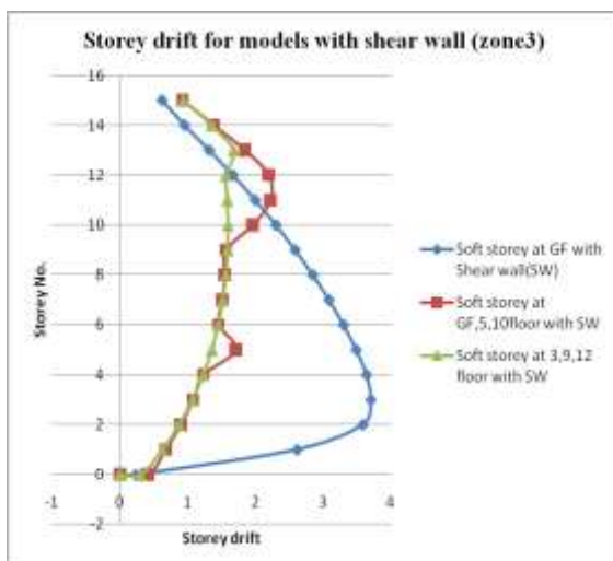
Fig.14: Storey drifts for models with Shear wall for zone3 in X-direction
