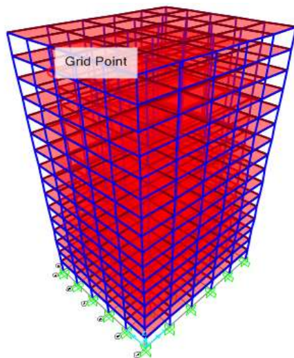
Fig 1. Bare frame model.
