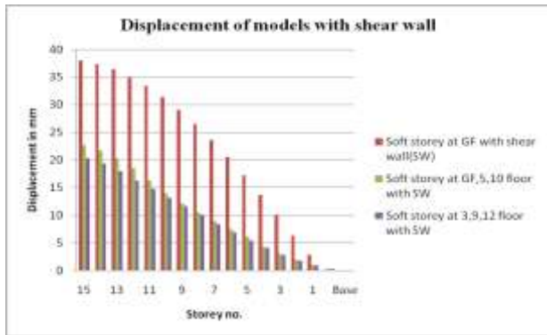
Fig 4: Graph of displacement of model with shear wall for Zone III in x direction.
