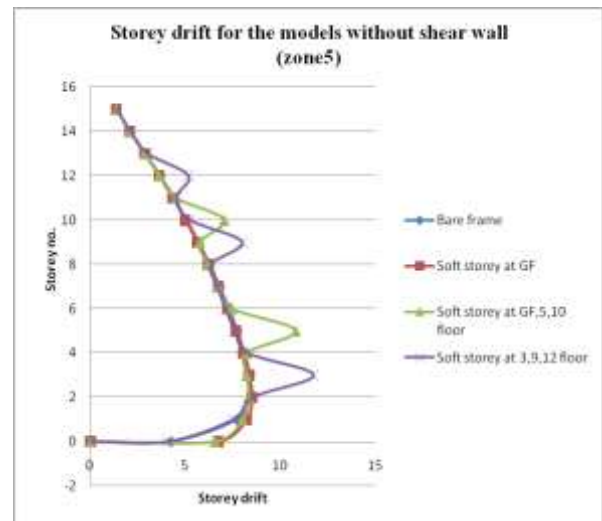
Fig.15: Storey drifts for models without Shear wall for zone5 in X-direction
