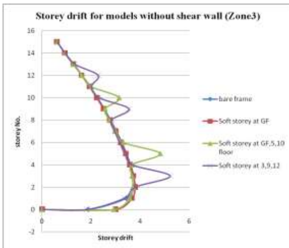
Fig.13: Storey drifts for models without Shear wall for zone3 in x-direction
