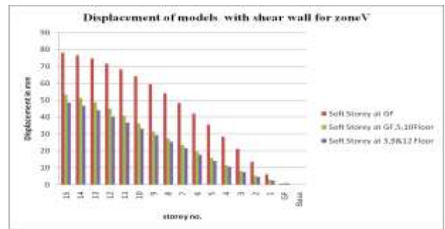
Fig 6: Graph of displacement of model with shear wall for Zone V in x direction.
