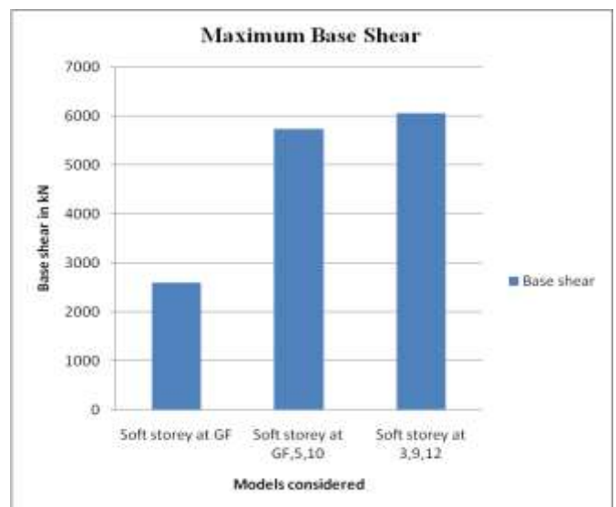
Fig 12. Base shear for models with shear wall in seismic zone V in x-direction.
