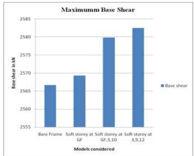
Fig 11. Base shear for models without shear wall in seismic zone V in x-direction.
