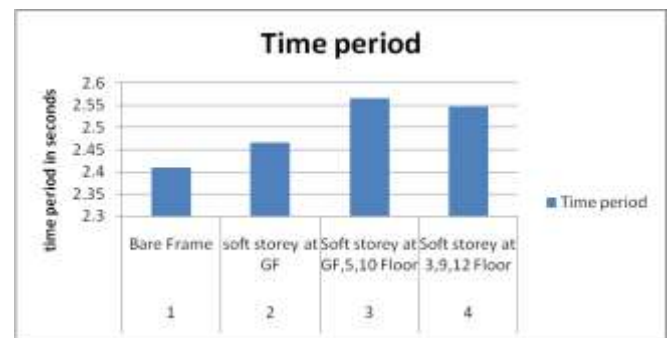
Fig 7: Graph of time period of models without shear wall for seismic zone III & V.
