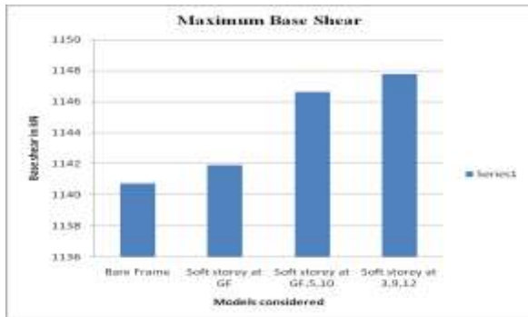
Fig 9. Base Shear for models without Shear wall in seismic zone III in x-direction.
