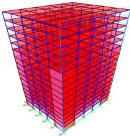
Fig 2. Model with soft storey and shear wall upto soft storey
