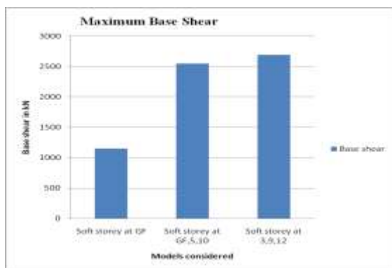
Fig 10. Base Shear for models with shear wall in seismic zone III in x-direction.
