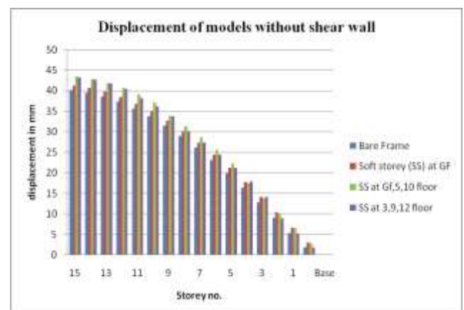
Fig 3: Graph of displacement of model without shear wall for Zone III in x direction.
