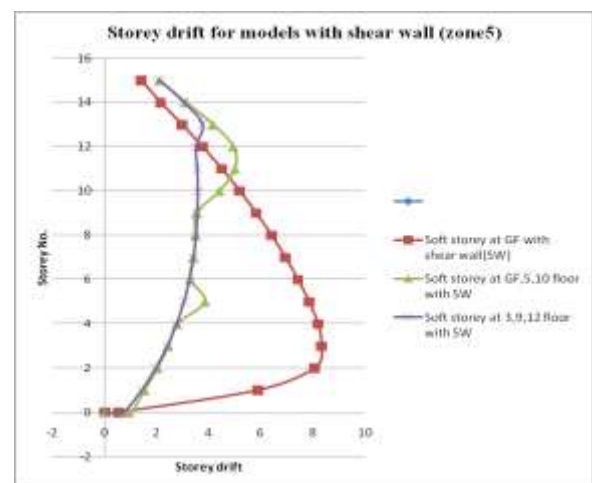
Fig.17: Storey drifts for models with Shear wall for zone5 in X-direction
