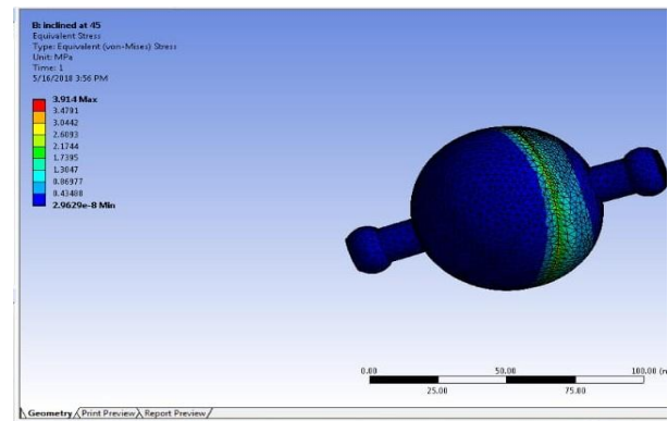
Fig. 11: Equivalent stress inclined spherical ball
