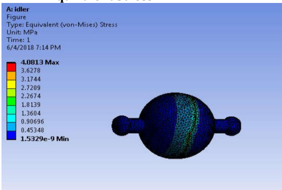
Fig. 8: Equivalent stress
