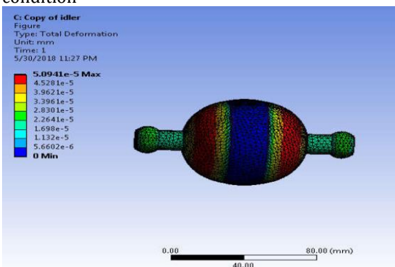
Fig. 9: total deformation under ideal running condition
