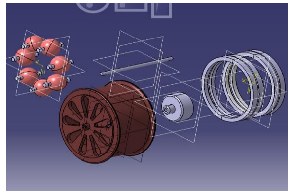
Fig. 6: Exploded view of planetary ball power transmitting system
