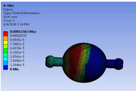
Fig. 7: total deformation of planetary ball when torque is high
