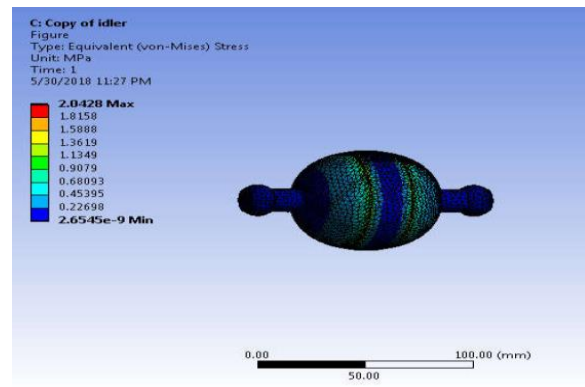
Fig. 10: Fixed equivalent stress.
