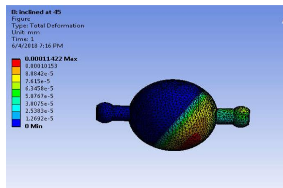
Fig. 12: Total deformation
