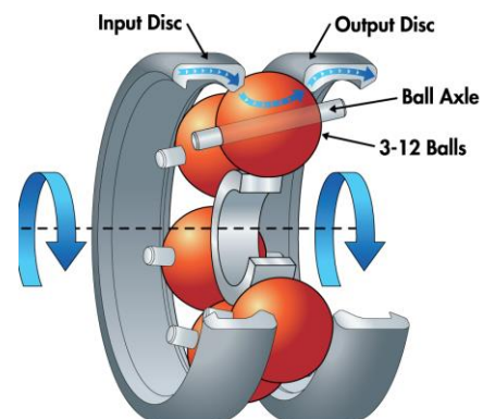
Fig. 1: working of planetary ball continuously variable transmission system
