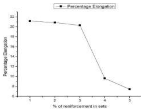
Fig. 4: Variation in Percentage elongation with weight fraction.
