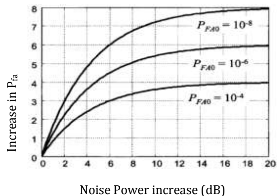
Figure 2.1: Increase in P_{fa} for a fixed threshold due to increase in \beta^2
