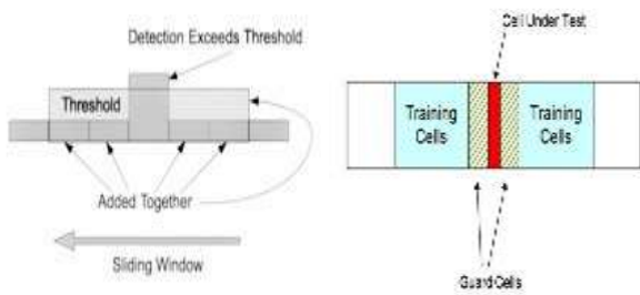
Figure 1.1: Cell - Averaging CFAR principle
