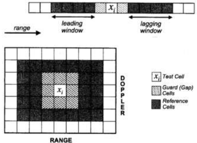
Figure 2.3: CFAR Windows. (a) 1-D Window for Range-Only Processor; (b) 2-D Window for Range-Doppler Processor
