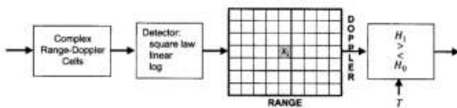
Figure 2.2: General radar detection processor
