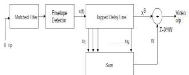
Figure 1.2: CA-CFAR receiver
