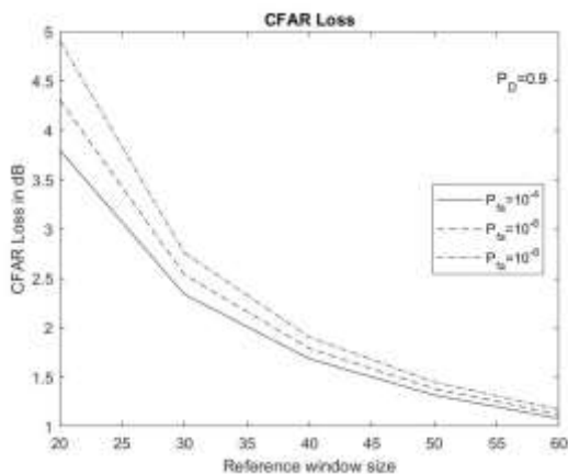
Figure 3.1: CA - CFAR loss for target in Gaussian interference with P_D = 0.9
