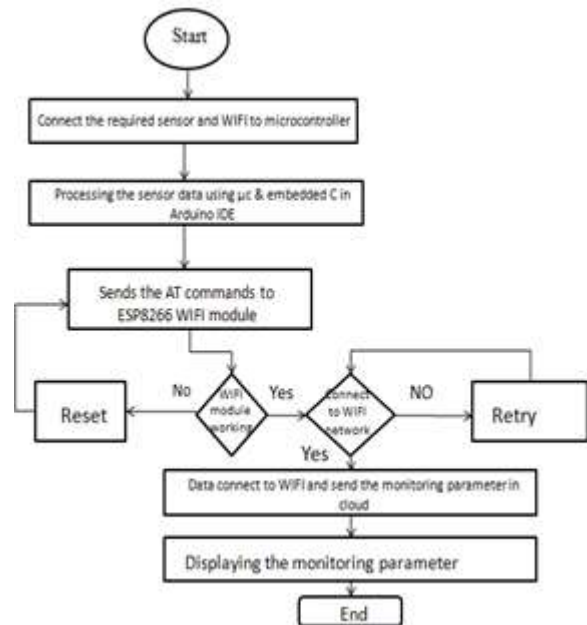
Fig.4-Process flow for sending meter status
