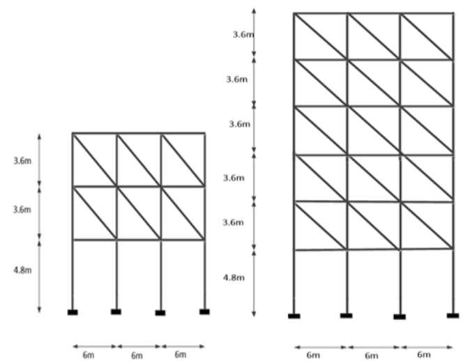
Fig.3: Elevation of three and six storey buildings with solid concrete block infill walls at the upper storey
