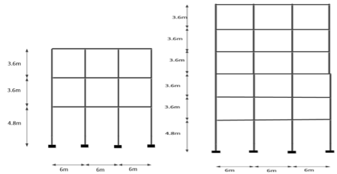
Fig.2: Elevation of three and six storey bare frame buildings
