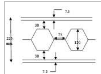
Figure No 5: Sample Considered For The Validation With WVS 225
