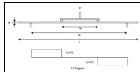
Figure No 6: Loading considered for WVS 225
