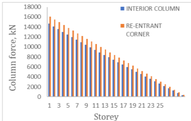
Chart -15: Column forces
