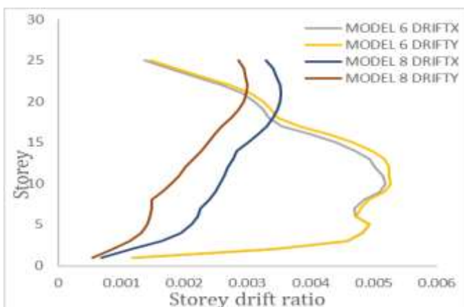
Chart -12: Storey drift ratio for M6 and M8
