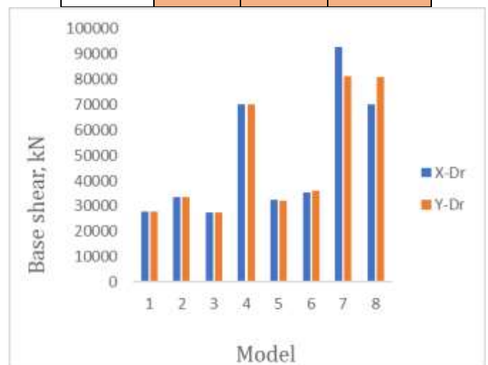
Chart -14: Base shear
