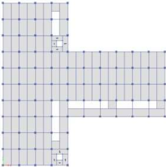
Fig -1: Plan view of T-shape structure without shear wall
