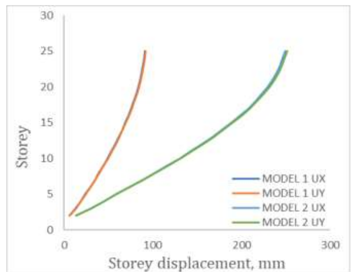
Chart -1: Storey displacement for M1 and M2
