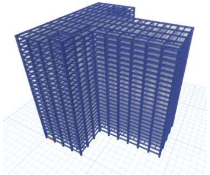
Fig-3: 3D view of T-shape structure without shear wall
