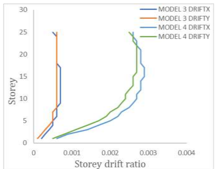
Chart -5: Storey drift ratio for M3 and M4
