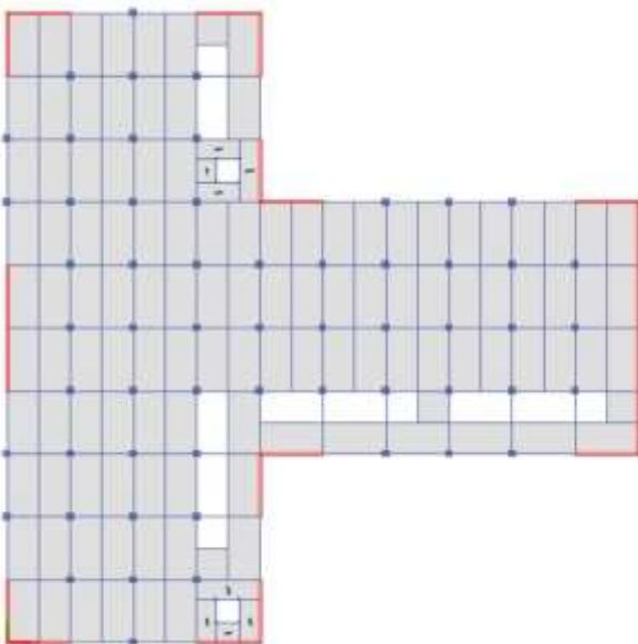
Fig-2: Plan view of T-shape structure with shear wall
