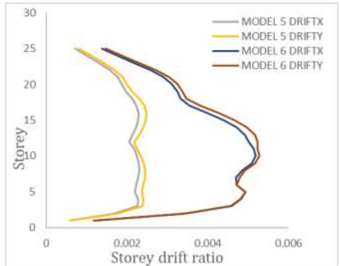
Chart -10: Storey drift ratio for M5 and M6
