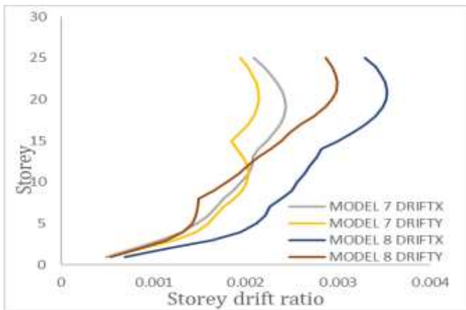
Chart -11: Storey drift ratio for M7 and M8
