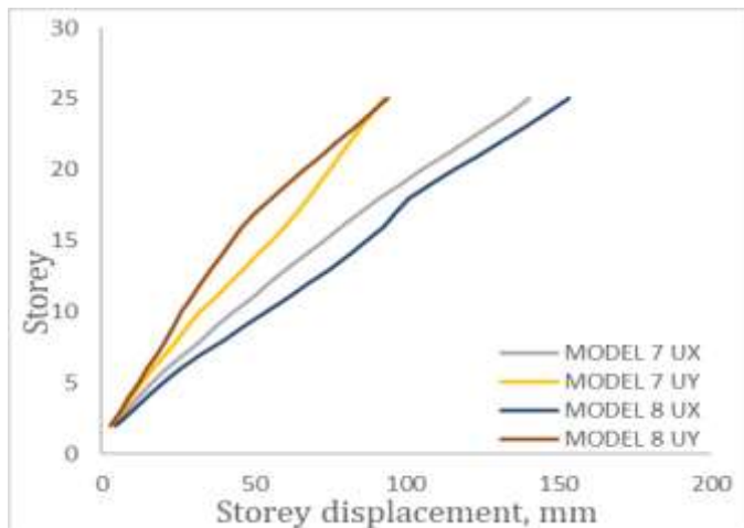
Chart -8: Storey displacement for M7 and M8
