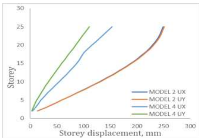
Chart -3: Storey displacement for M2 and M4
