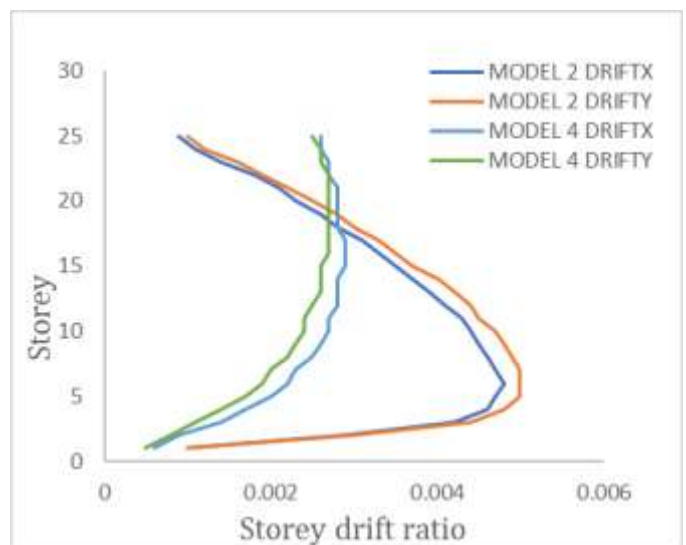
Chart -6: Storey drift ratio for M2 and M4
