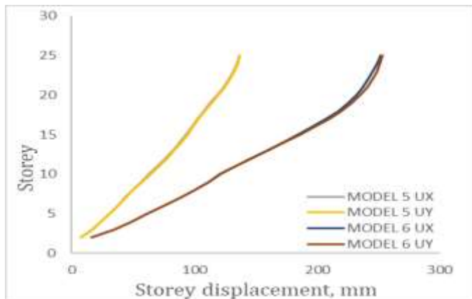
Chart -7: Storey displacement for M5 and M6
