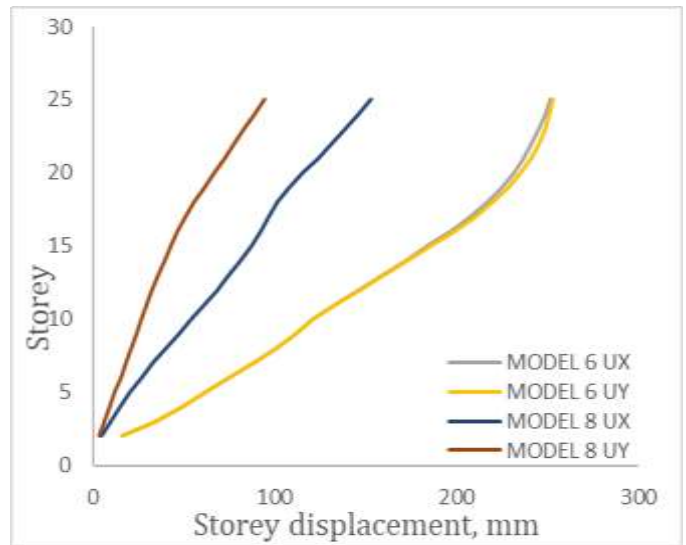
Chart -9: Storey displacement for M6 and M8
