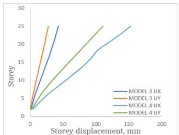
Chart -2: Storey displacement for M3 and M4
