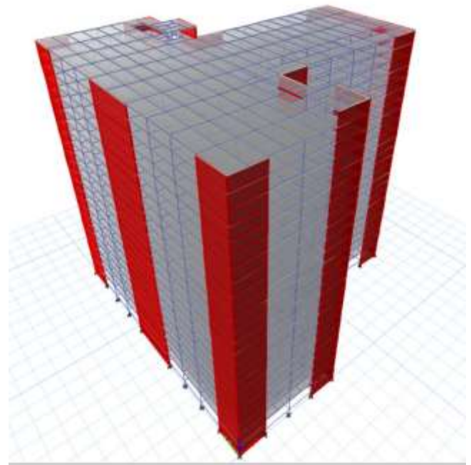
Fig-4: 3D view of T-shape structure with shear wall
