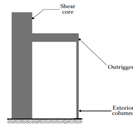
Fig. 3.11 offset core with outrigger and belt wall structure
