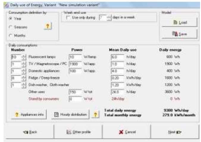
Fig - 9: Household load consumption
