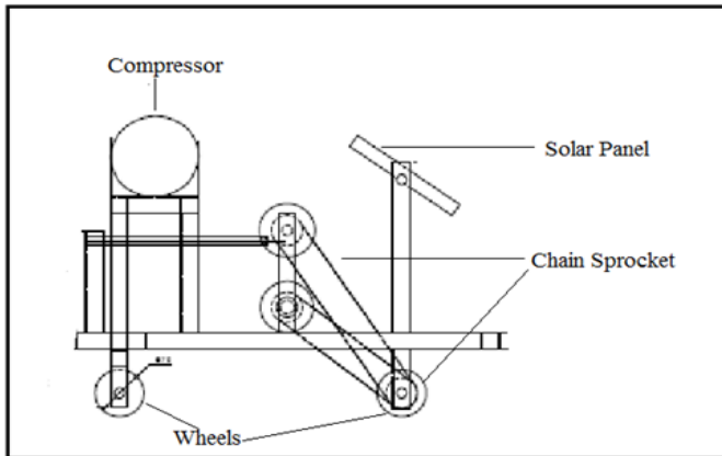
Fig -1: Block diagram of Water Sprinkling Robot
