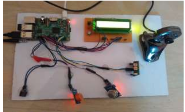
Fig -6: Experimental Setup
