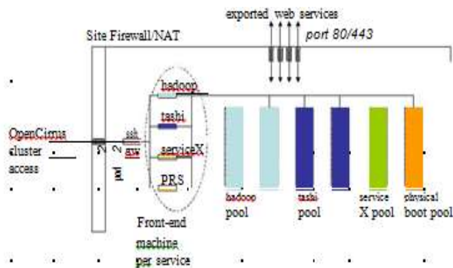
Figure 4. A typical Open Cirrus site.
