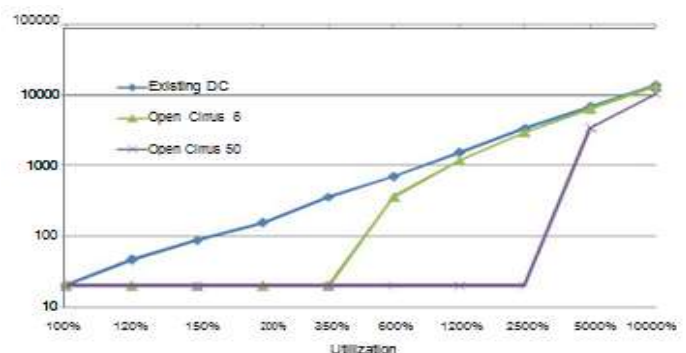
Figure 5. Overload Under-provisioned Site to AWS v. 6/50 Sites
