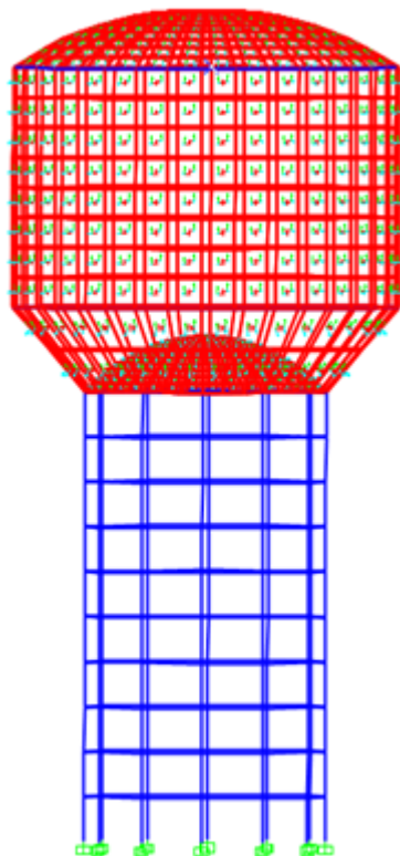
SAP 2000 MODEL FOR INTZE TANK WITH SHAFT STAGING
