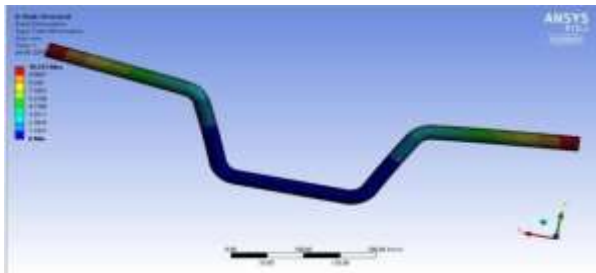
Fig: 3.2.-Structural Analysis (For Ref. only)
