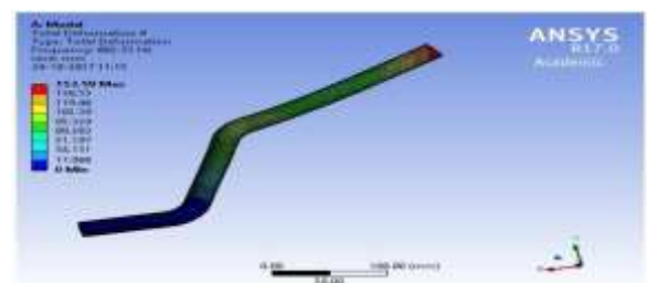
Fig: 3.1-Modal Analysis (For Ref. only)
