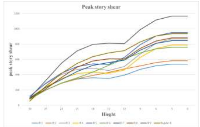
Chart - 1: Peak story shear
