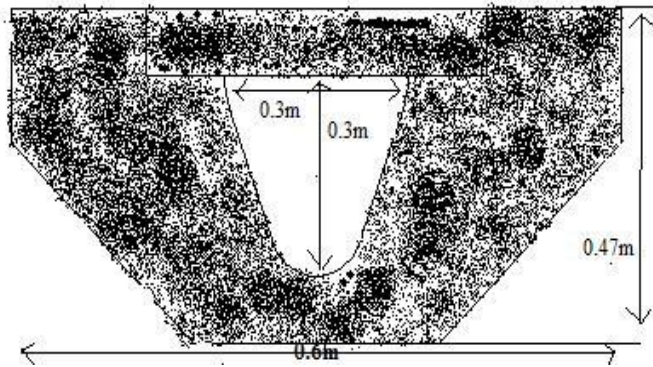
Fig-3: Design of Gutter
