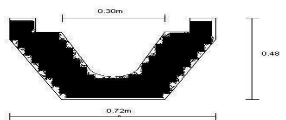
Fig -10: Dimensions of Gutter
