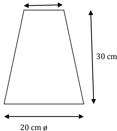
Fig 4.1: Slump apparatus
