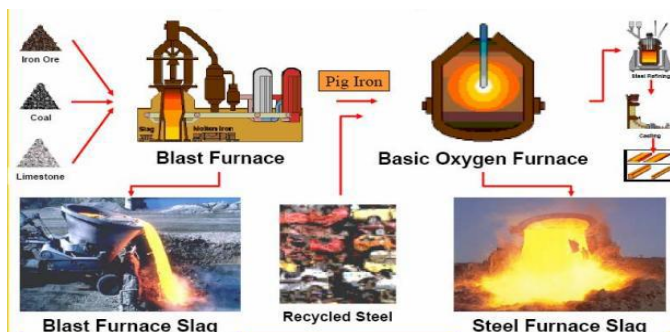
Fig.2 Production of Steel Slag
