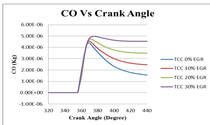
Fig.12. CO emissions at different percentage of EGR
