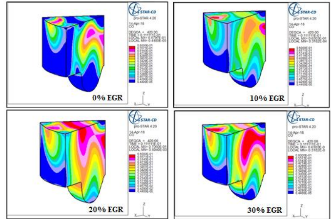
Fig.13. CO contour at 420 degrees for different percentage of EGR
