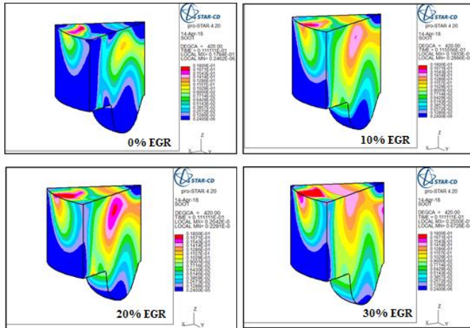
Fig.11. soot emission contour at 420 degrees for different percentage of EGR
