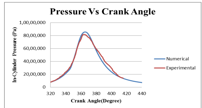
Fig.5. Validation between numerical and experimental graphs
