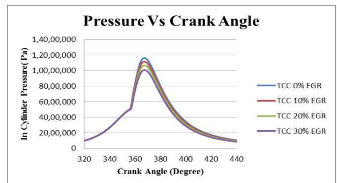
Fig.6. Cylinder pressure with respect to crank angle at different percentage of EGR
