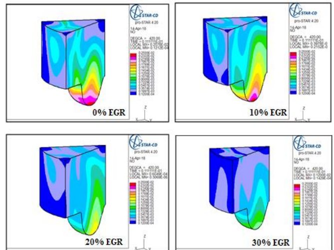
Fig.9. NOx contour at 420 degree crank angle at different percentage of EGR
