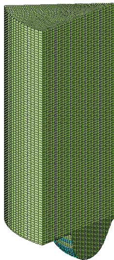
Fig -4: Computational grids at 100° before TDC
