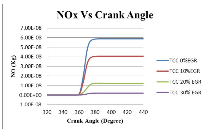
Fig.8. NOx emissions with respect to crank angle at different percentage of EGR
