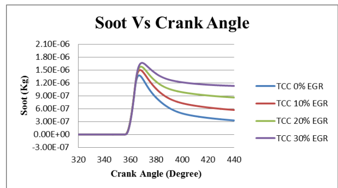
Fig.10. soot emissions at different percentage of EGR
