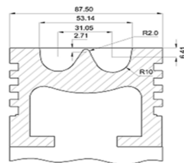
Fig -1. Dimensions of the TCC geometry
