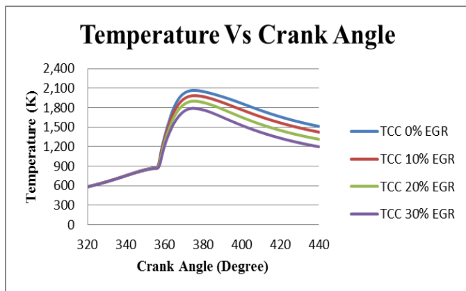
Fig.7. Cylinder temperatures with respect to crank angle at different percentage of EGR
