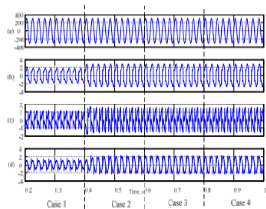
Fig.8.Simulation result: (a) grid voltage, v_s v,(b) load current, i_L ,A(c) inverter current, i_{sat} (A),and (d)grid current, i_g ,A.
