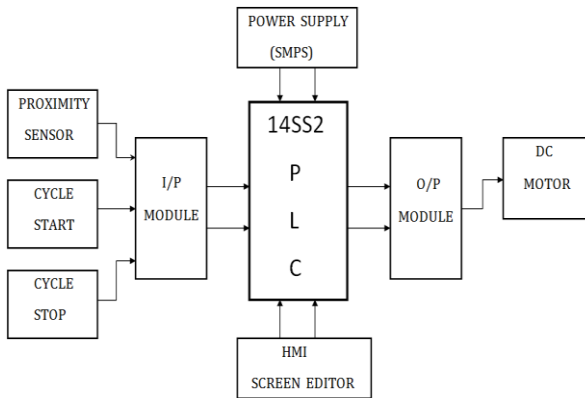
Fig -1: Block diagram of Advanced vehicle parking
