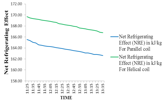
Chart -1: NRE For parallel Vs Helical coil condenser
