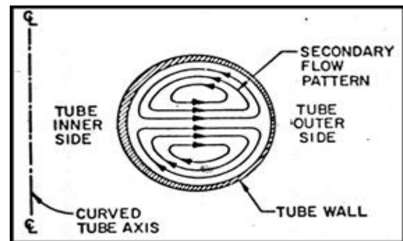
Fig: 1.1 Sketch of secondary flow pattern in curved tube
