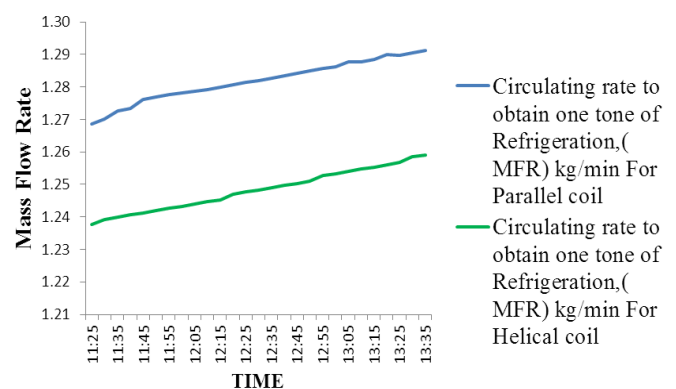
Chart -2: Mass Flow Rate For parallel Vs Helical coil condenser
