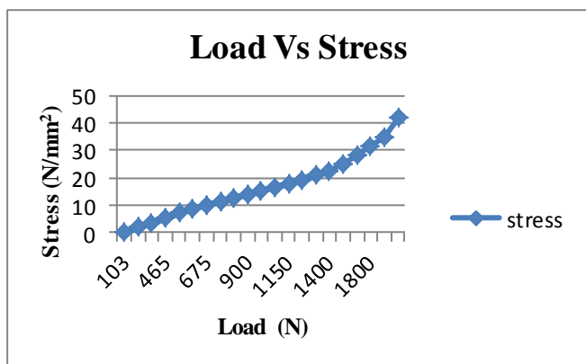
Fig. 6 Load Vs stress graph of FEA result.
