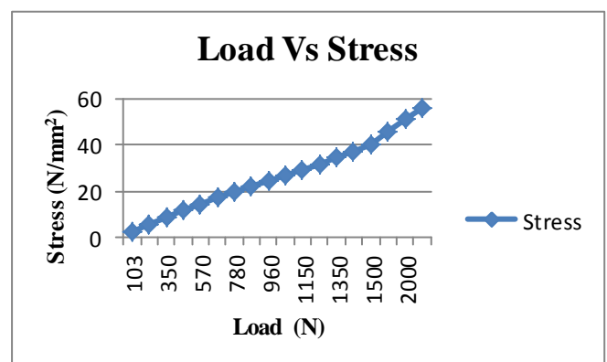
Fig. 8 Load Vs Stress graph from experimental method for Al 6063.
