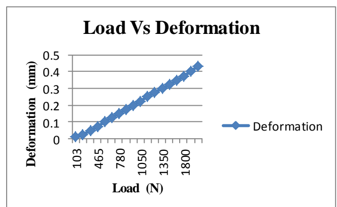
Fig. 7 Load Vs deformation graph from experimental method for Al 6063.
