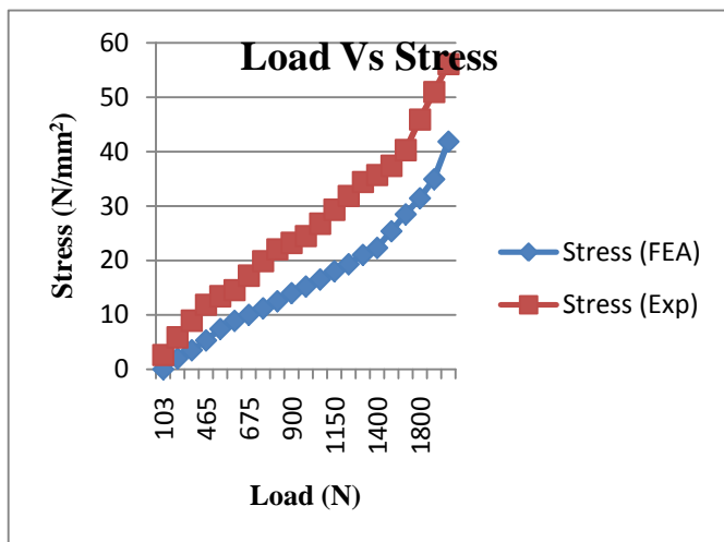
Fig. 10 Comparison Graph of Load Vs Stress graph by FEA and experimental method.
